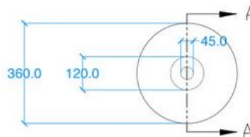
Underside View
