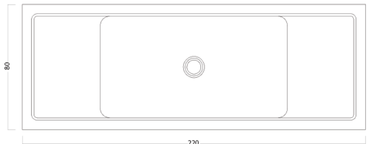
PLAN VIEW
